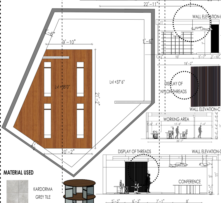
REFLECTED FALSE CEILING
