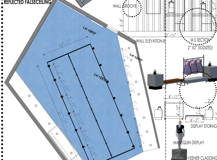
REFLECTED FALSECEILING
