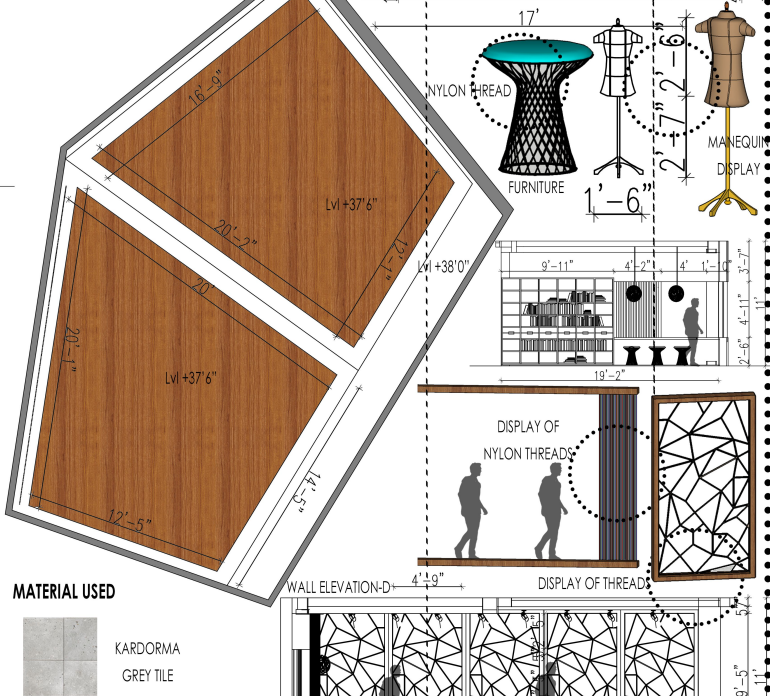
REFLECTED FALSE CEILING
