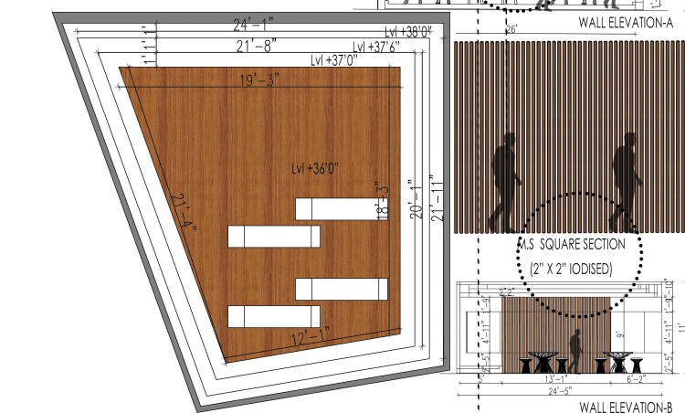
REFLECTED FALSE CEILING
