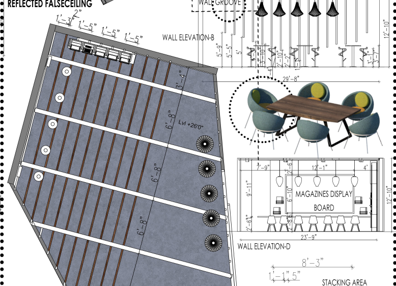
REFLECTED FALSECEILING
